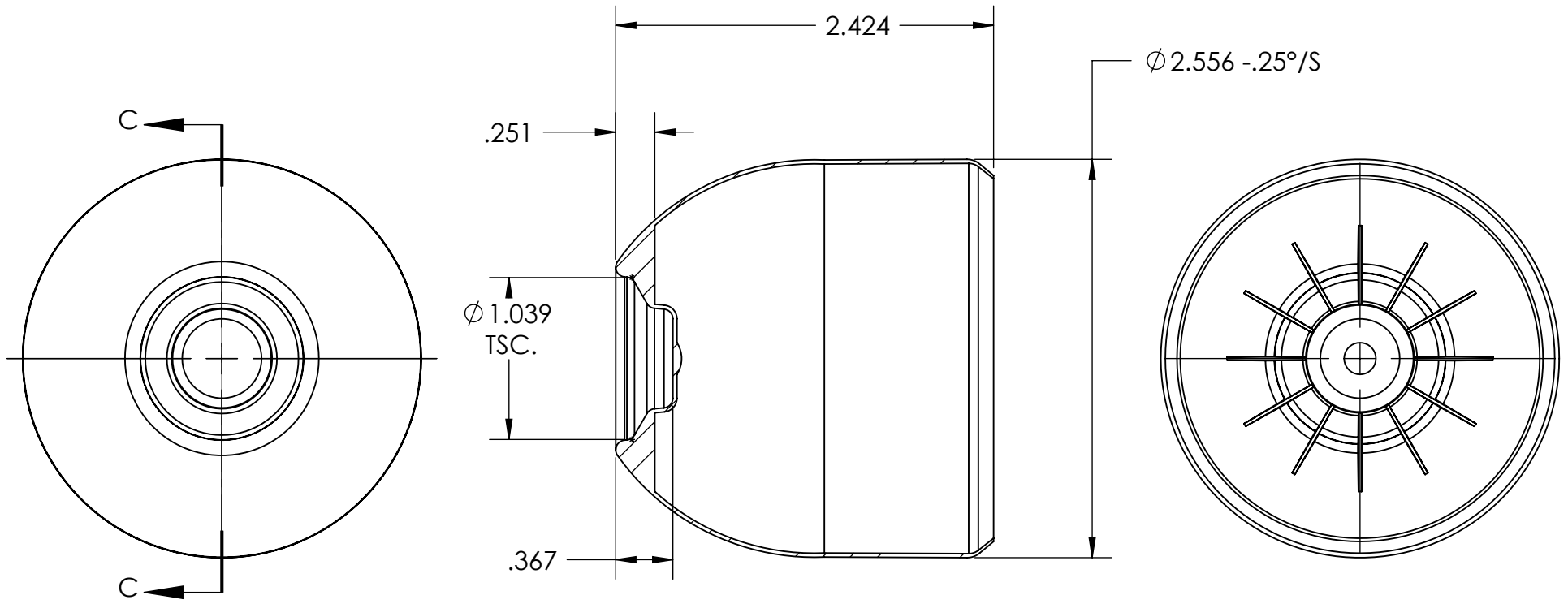
SECTION C-C
