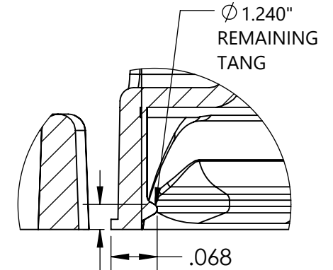
DETAIL J SCALE 5 : 1
