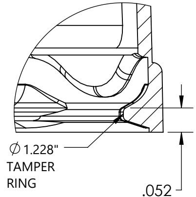
DETAIL K SCALE 5 : 1
