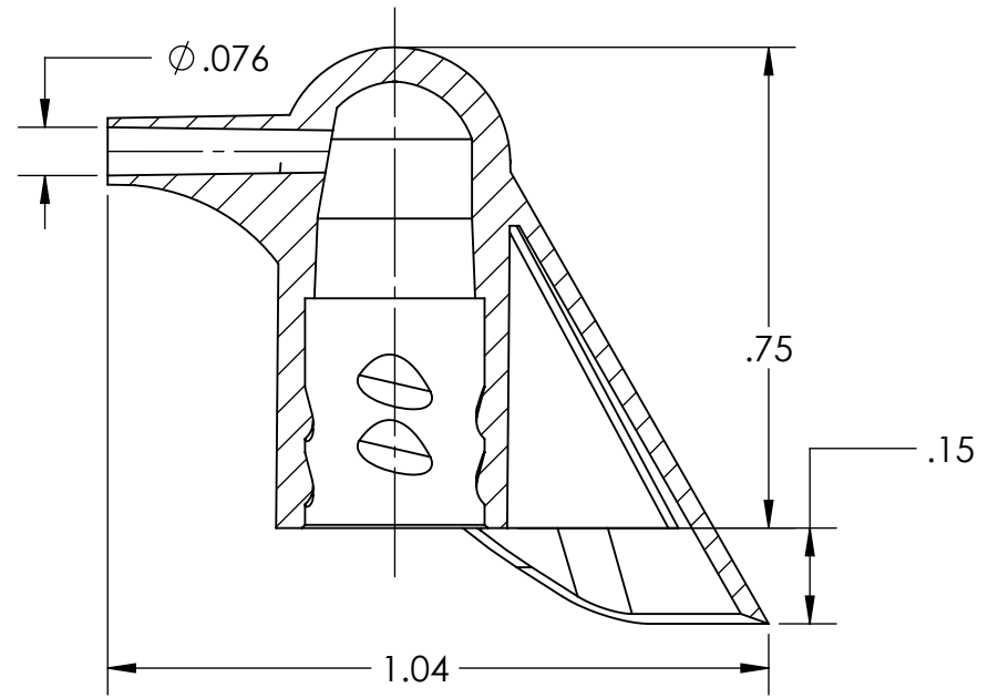
SECTION H-H
